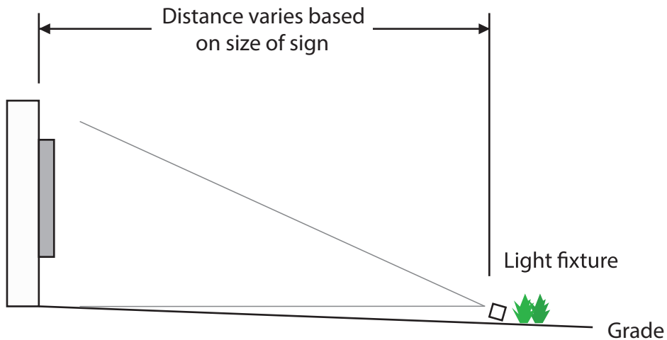
Side view of sign panel with logo sign
